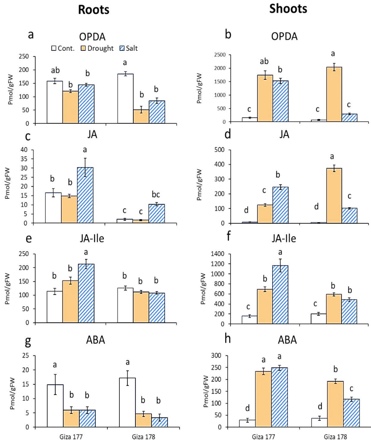
Figure 6. The level of jasmonates (OPDA, JA, and JA-Ile) and ABA under control and 1 day of drought and salinity in both roots and shoots of rice seedling exposed to drought and salinity. a and b 12-oxyphytodenic acid (OPDA), c and d: Jasmonic acid (JA), e and f JA-isoleucine (JA-Ile), g and h: abscisic acid (ABA). Values represent the mean of at least three independent experiments \pm SE. Significant differences amongst different treatments are indicated by different letters, according to Tukey's Honest Significant Difference (HSD) test ( P < 0.05 ).
