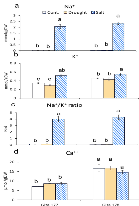
Figure 2. Sodium (a), potassium (b), sodium/potassium ratio (c) and calcium (d) ions contents in shoots in rice seedlings subjected to drought (mannitol) and salinity (NaCl). Values represent the mean of at least three independent experiments \pm SE. Significant differences amongst different treatments are indicated by different letters, according to Tukey's Honest Significant Difference (HSD) test ( P < 0.05 ).
