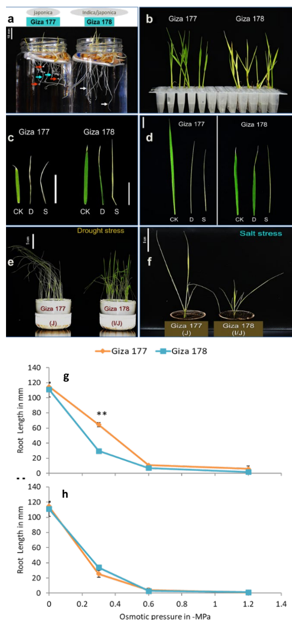
Figure 1. Phenotypic response of Giza 177 and Giza 178 to control (CK), drought (D), and salt stress (S). a root coiling phenotype in Giza 177 compared to straightened roots of Giza 178 (indica/japonica) under control conditions in light, red arrows point at totally coiled roots, blue arrows point at curly roots (both in Giza 177), and white arrows for straightened roots in Giza 178. b phenotyping of nitrogen deficiency symptoms appeared with Giza 178 (leaves yellowing and chlorosis) compared to Giza 177 with more greenish and healthy leaves. Phenotyping of the second leaves (c) and the third leaves (d) of Giza 177 and Giza 178 with mannitol-simulated drought and NaCl-simulated salt stress (scale bar equals to 1 cm). e phenotyping of Giza 177 and Giza 178 in response to drought triggered by holding irrigation for 5 days in sandy soil containers. f phenotyping of Giza 177 and Giza 178 in response to saline irrigation of 100 mM NaCl. Root length assay of Giza 177 and Giza 178 under different levels of osmotic potentials (0, -0.3, -0.6, and -1.2 MPa) of mannitol (g) and NaCl (h). **significant difference at P < 0.01 in a student's t-test.
