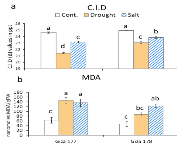
Figure 3. Carbon Isotope Discrimination (C.I.D or \Delta ) as readout for stomatal aperture (a), and lipid peroxidation as readout for oxidative damage (b). Values represent the mean of at least three independent experiments \pm SE. Significant differences amongst different treatments are indicated by different letters, according to Tukey's Honest Significant Difference (HSD) test ( P < 0.05 ).
