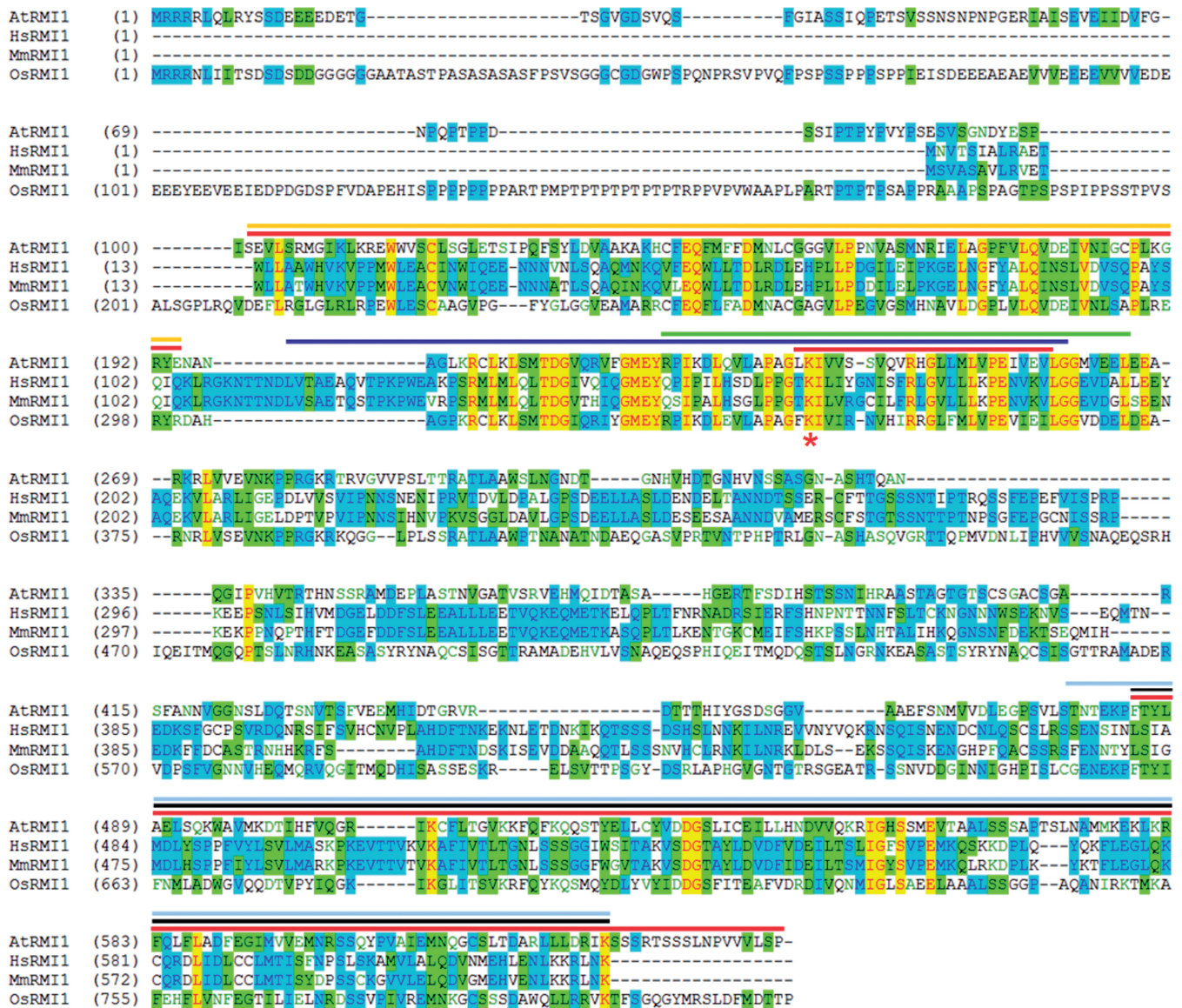
Figure 1. Alignment of RMI1 homologues from A. thaliana , Homo sapiens , Mus musculus and Oryza sativa . Identical amino acids for all four proteins are highlighted in yellow and for three proteins in blue. Similar amino acids are highlighted in green. The sequence regions that were deleted in the respective AtRMI1 variants are marked in red ( \Delta DUF: aa 101–194; \Delta OB1: aa 234–258; \Delta OB2: aa 485–644). The yellow overlined region in the N-terminus indicates the conserved DUF1767 domain [pfam08585; (25)]. The subsequent blue overlined sequence highlights the putative OB-fold domain 1 of HsRMI1, as described by Yin et al. (17). The green overlined amino acid region has been shown to be essential for the binding of HsBLM and HsTOP3A. Within the OB-fold domain 1, the conserved lysine (marked by an asterisk) has been described as an essential amino acid for interaction with HsTOP3A (30). The OB-fold domain 2 is located in the C-terminal part of RMI1 [overlined in black; (25)]. The OB-fold domain 2 of HsRMI1 is required for its interaction with HsRMI2.
