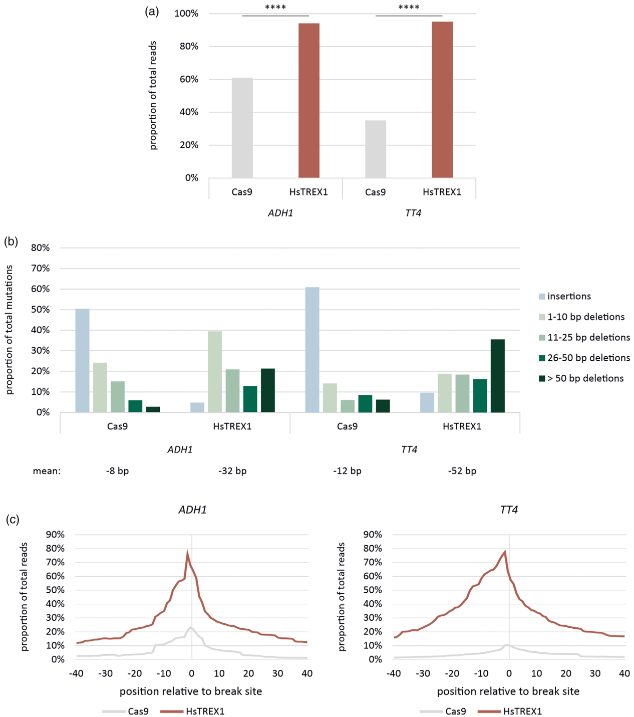
Figure 5. Validation of target-independent effects of SunTag-mediated HsTREX1 recruitment.
